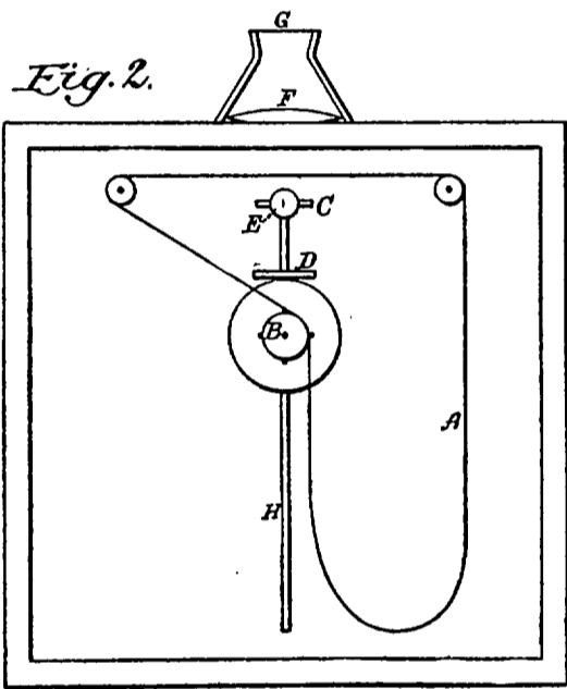
JENKINS' EARLY FORM OF CABINET—INTERMITTENT ILLUMINATION.
